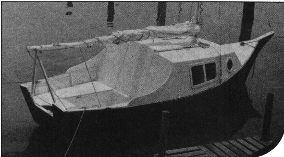
Completed boat showing cockpit, sliding hatch and the companionway door.
