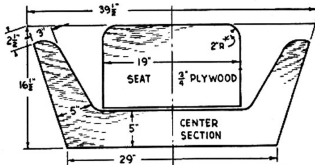
SEAT AND CENTER SECTION ARE CUT FROM ONE PIECE OF 3/4" PLYWOOD
