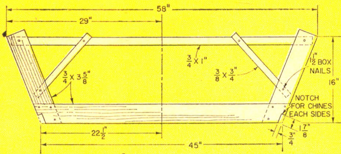
A MOLD FRAME
