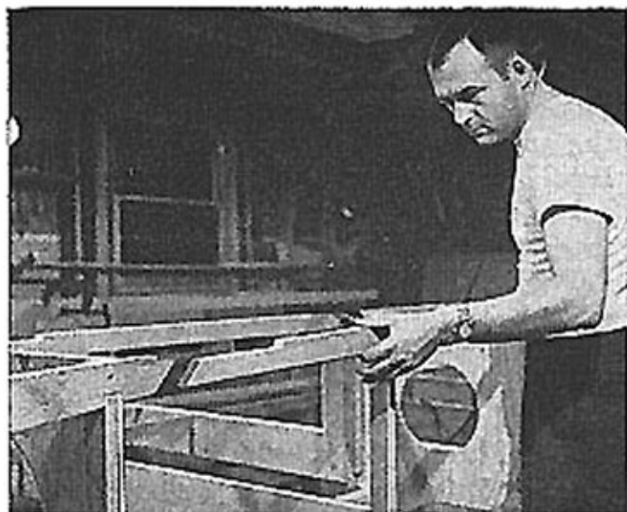
CHINE LOG JOINTS fall under joints in bottom planking and must be notched for \frac{3}{8} -in. butt plates
